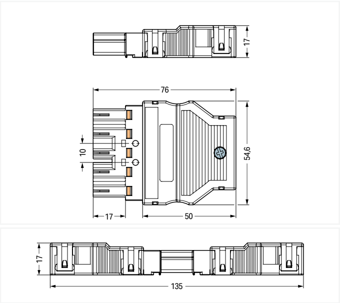
Overall length when mated Item-Specific Accessories
