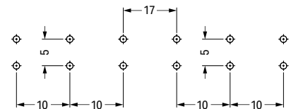
Angled design
