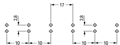
Straight design
