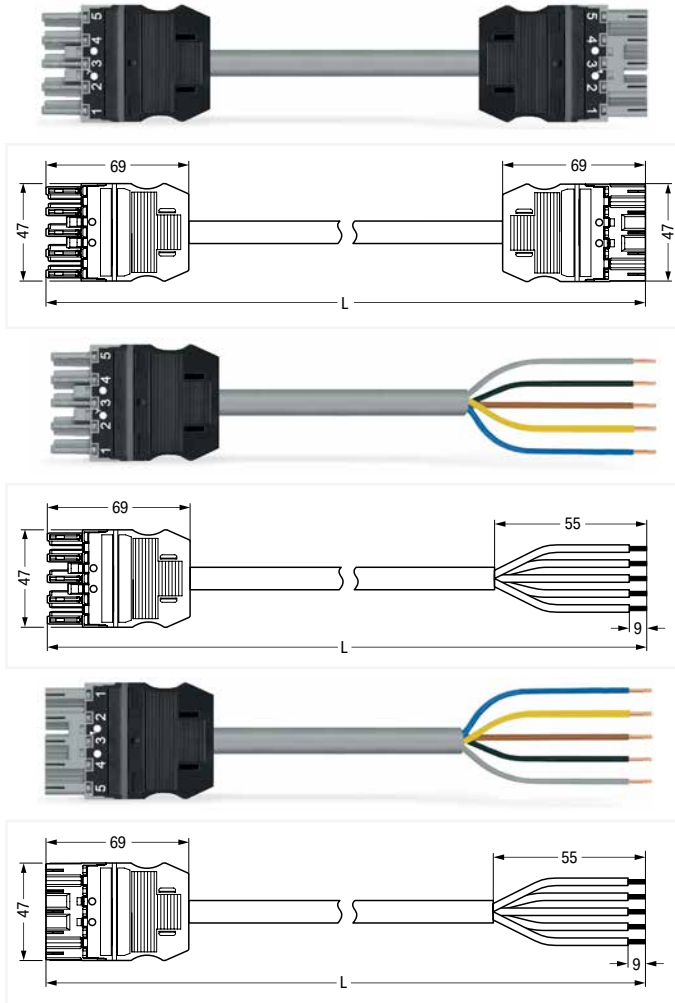
Interconnecting cable ► Socket - Plug
